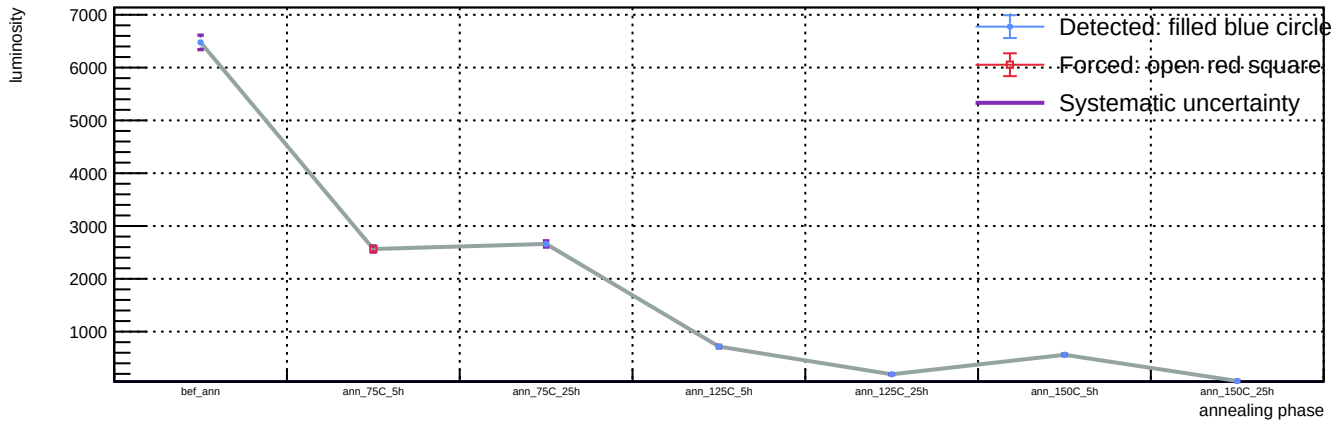
Sensor B1, v = 3 V, representative T = 23 C (max available) - Spot 14: luminosity vs phase
