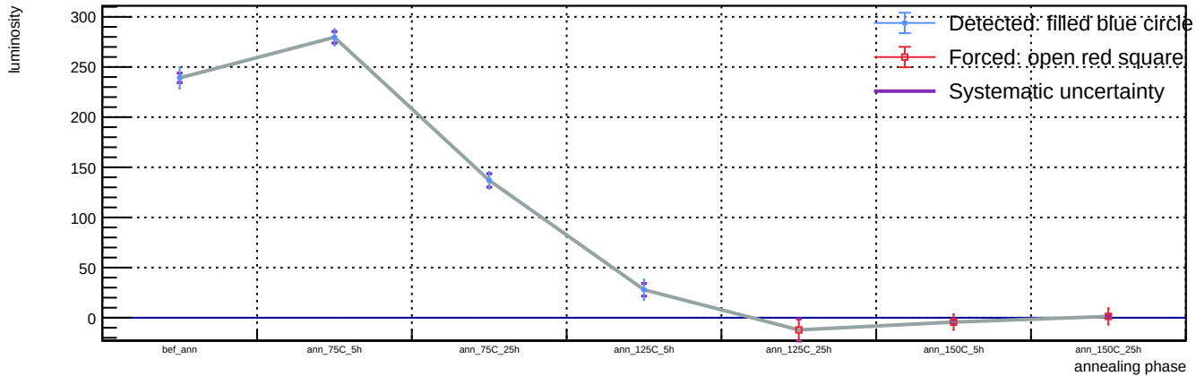
Sensor B1, v = 3 V, representative T = 23 C (max available) - Spot 17: luminosity vs phase
