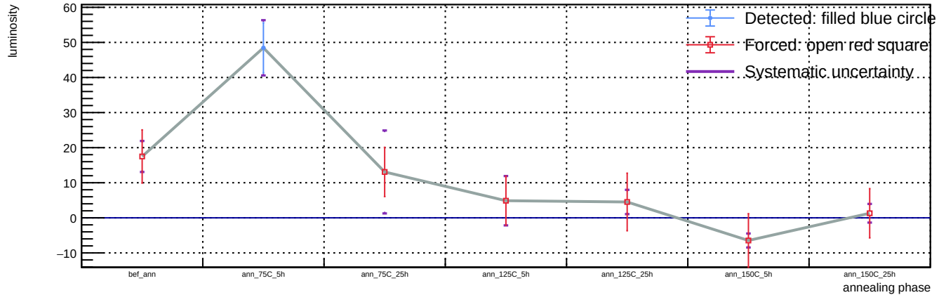
Sensor B1, v = 3 V, representative T = 23 C (max available) - Spot 24: luminosity vs phase
