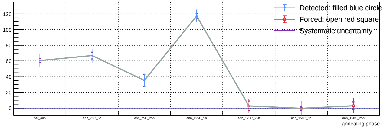
Sensor B1, v = 3 V, representative T = 23 C (max available) - Spot 28: luminosity vs phase
