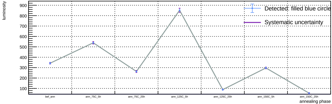
Sensor B1, v = 3 V, representative T = 23 C (max available) - Spot 29: luminosity vs phase
