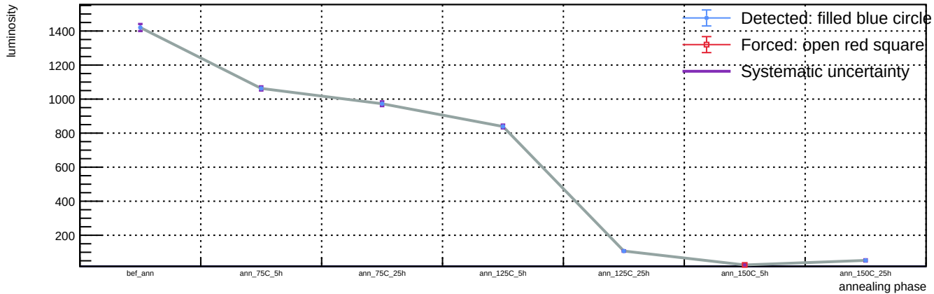
Sensor B1, v = 3 V, representative T = 23 C (max available) - Spot 36: luminosity vs phase
