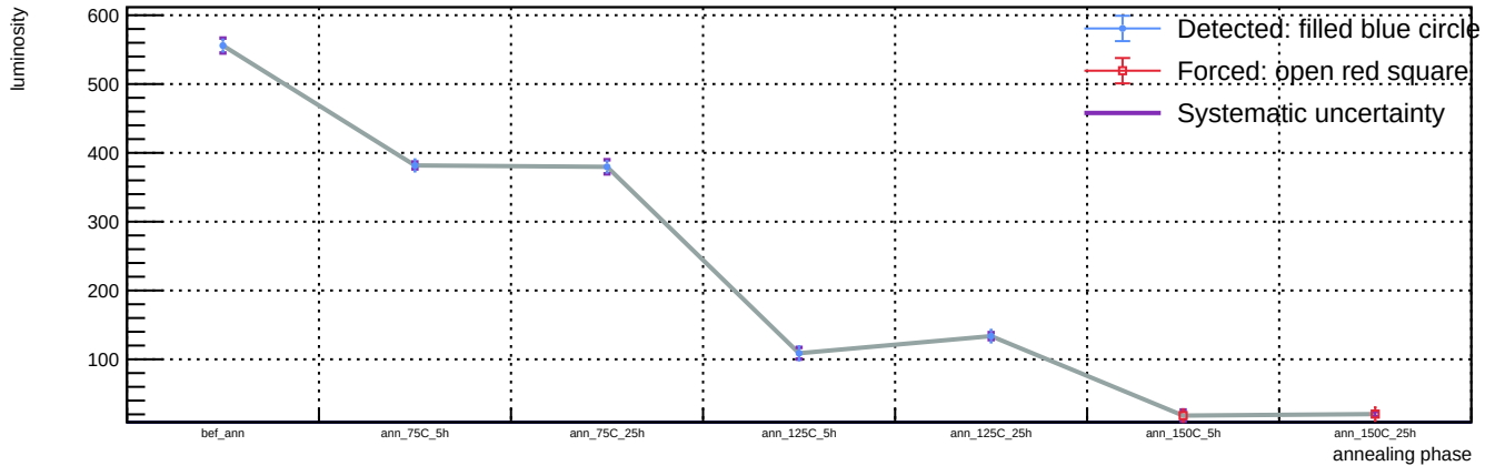
Sensor B1, v = 3 V, representative T = 23 C (max available) - Spot 42: luminosity vs phase
