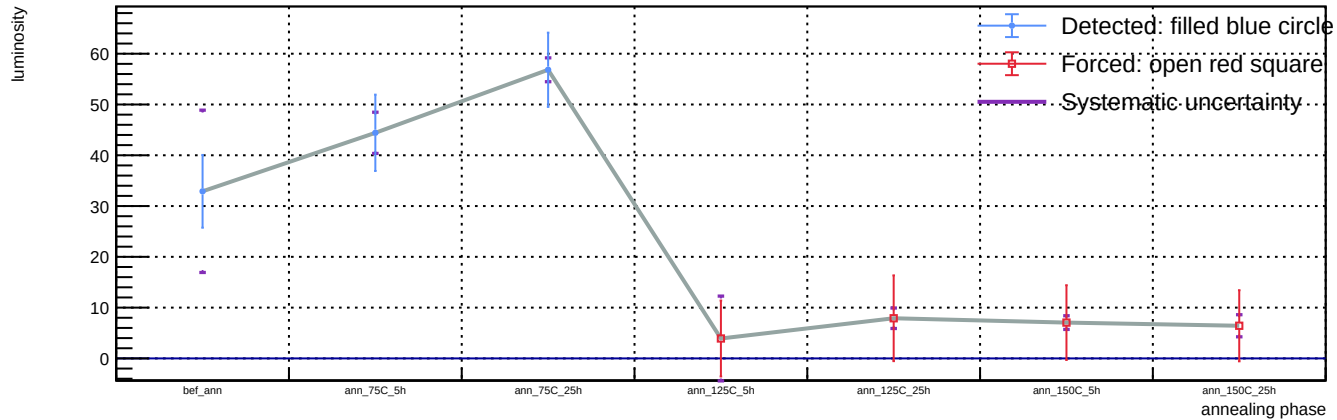
Sensor B1, v = 3 V, representative T = 23 C (max available) - Spot 47: luminosity vs phase
