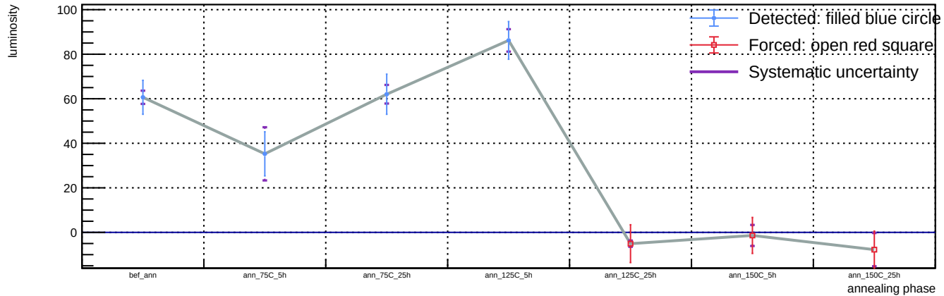
Sensor B1, v = 3 V, representative T = 23 C (max available) - Spot 48: luminosity vs phase
