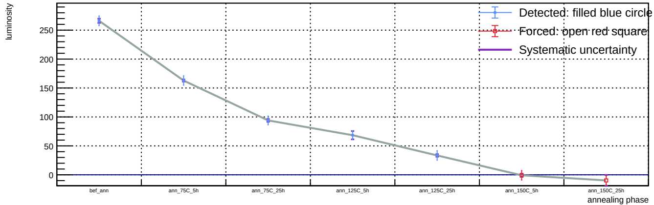
Sensor B1, v = 3 V, representative T = 23 C (max available) - Spot 5: luminosity vs phase
