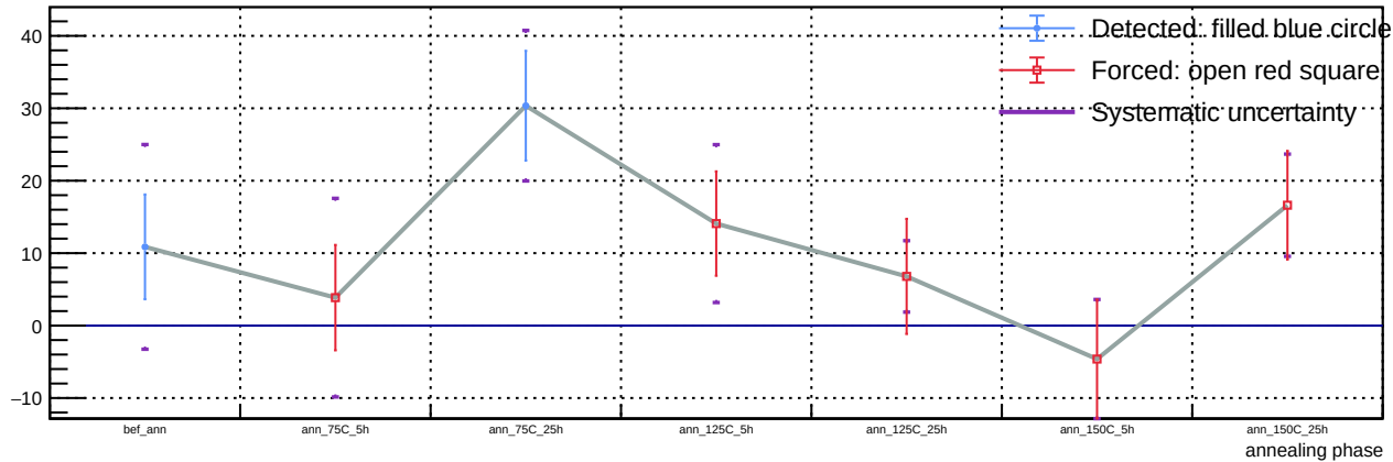
Sensor B1, v = 3 V, representative T = 23 C (max available) - Spot 54: luminosity vs phase
