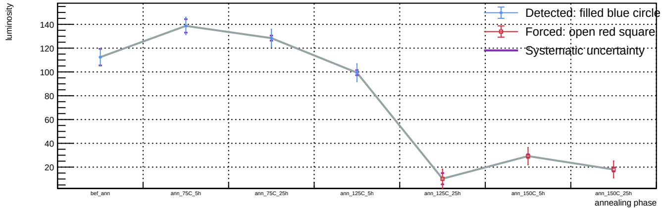
Sensor B1, v = 3 V, representative T = 23 C (max available) - Spot 58: luminosity vs phase
