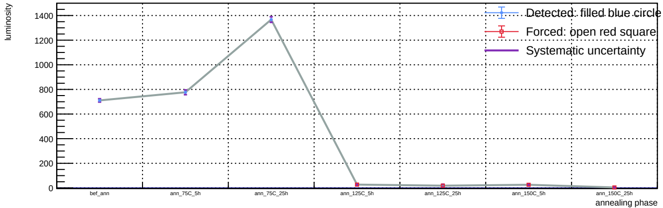
Sensor B1, v = 3 V, representative T = 23 C (max available) - Spot 59: luminosity vs phase
