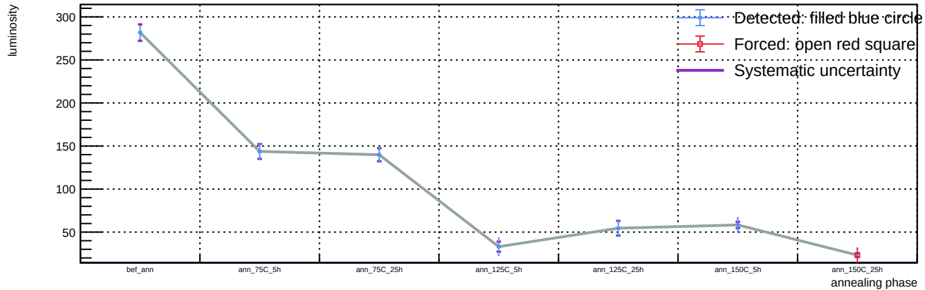
Sensor B1, v = 3 V, representative T = 23 C (max available) - Spot 61: luminosity vs phase
