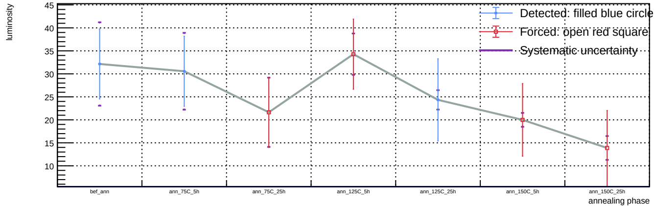
Sensor B1, v = 3 V, representative T = 23 C (max available) - Spot 7: luminosity vs phase
