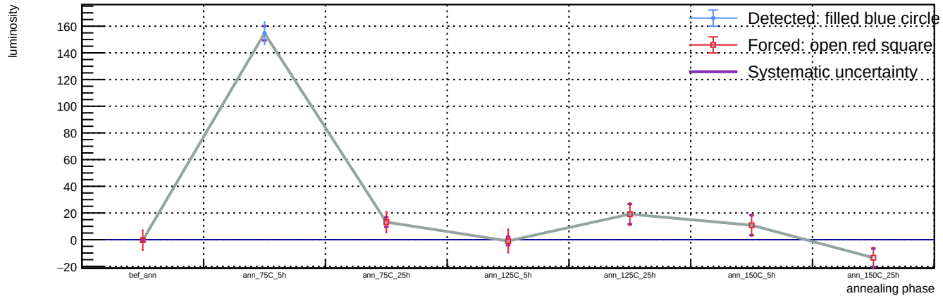
Sensor B1, v = 3 V, representative T = 23 C (max available) - Spot 71: luminosity vs phase
