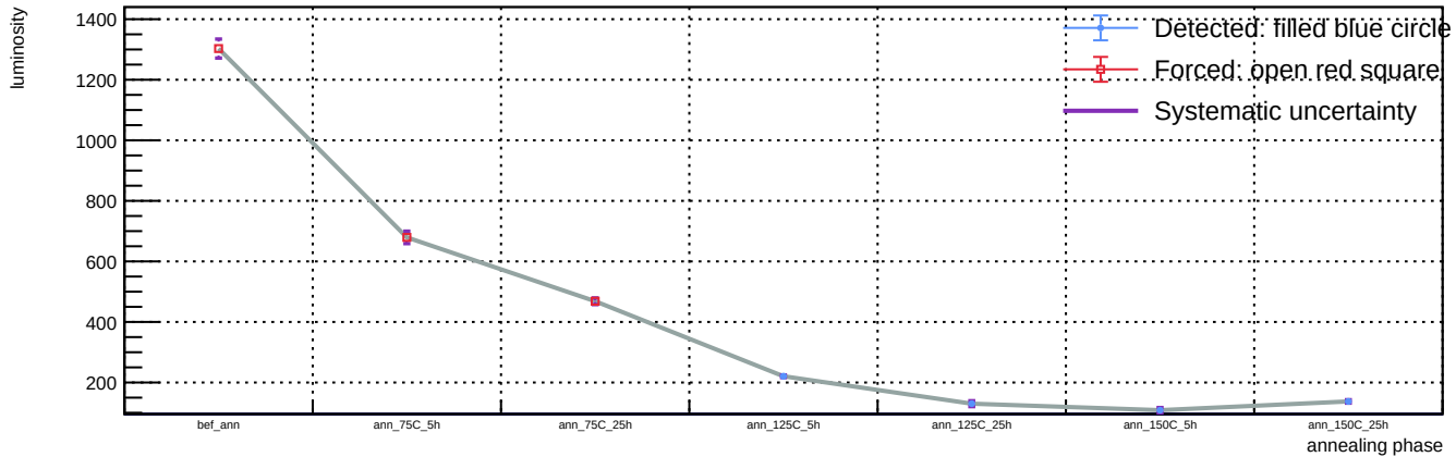
Sensor B1, v = 3 V, representative T = 23 C (max available) - Spot 85: luminosity vs phase
