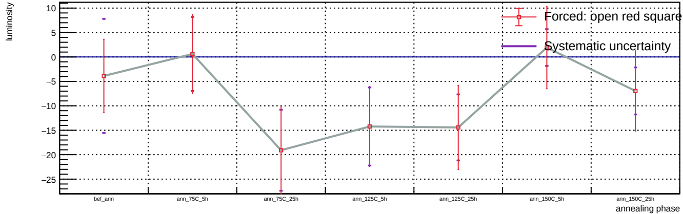
Sensor B1, v = 3 V, representative T = 23 C (max available) - Spot 86: luminosity vs phase
