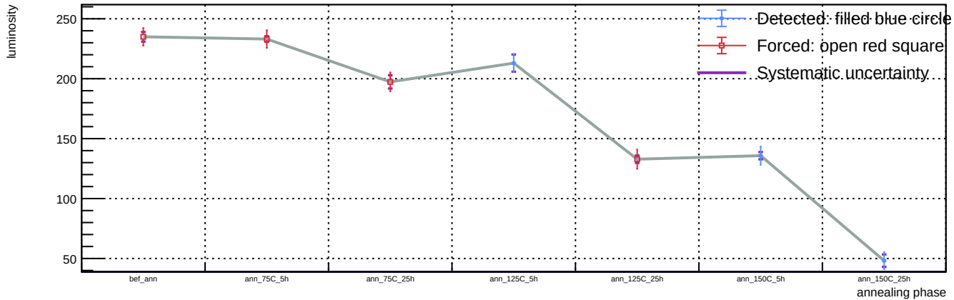
Sensor B1, v = 3 V, representative T = 23 C (max available) - Spot 91: luminosity vs phase
