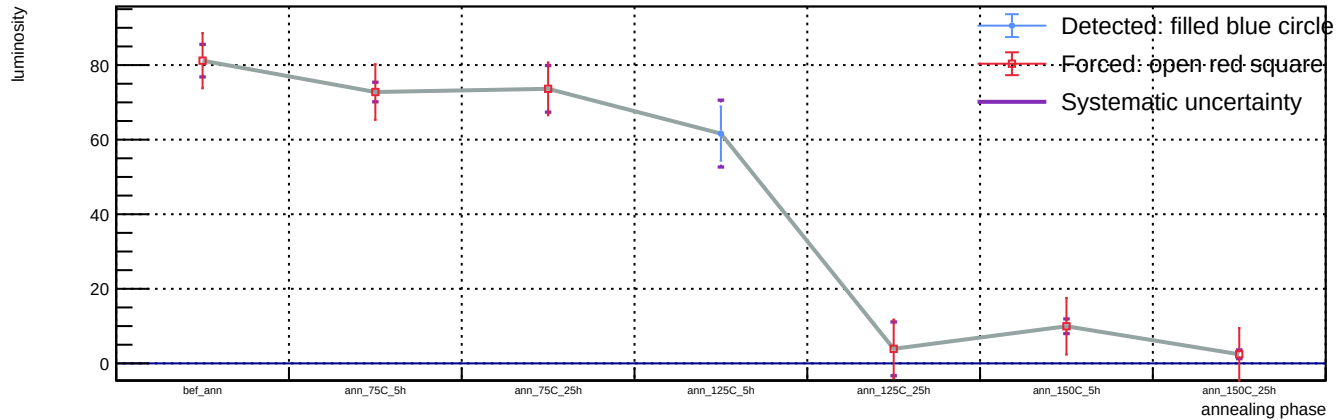
Sensor B1, v = 3 V, representative T = 23 C (max available) - Spot 96: luminosity vs phase
