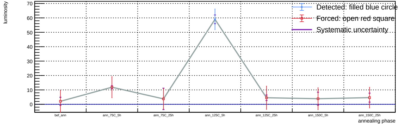
Sensor B1, v = 3 V, representative T = 23 C (max available) - Spot 97: luminosity vs phase
