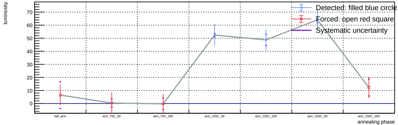
Sensor B1, v = 3 V, representative T = 23 C (max available) - Spot 98: luminosity vs phase
