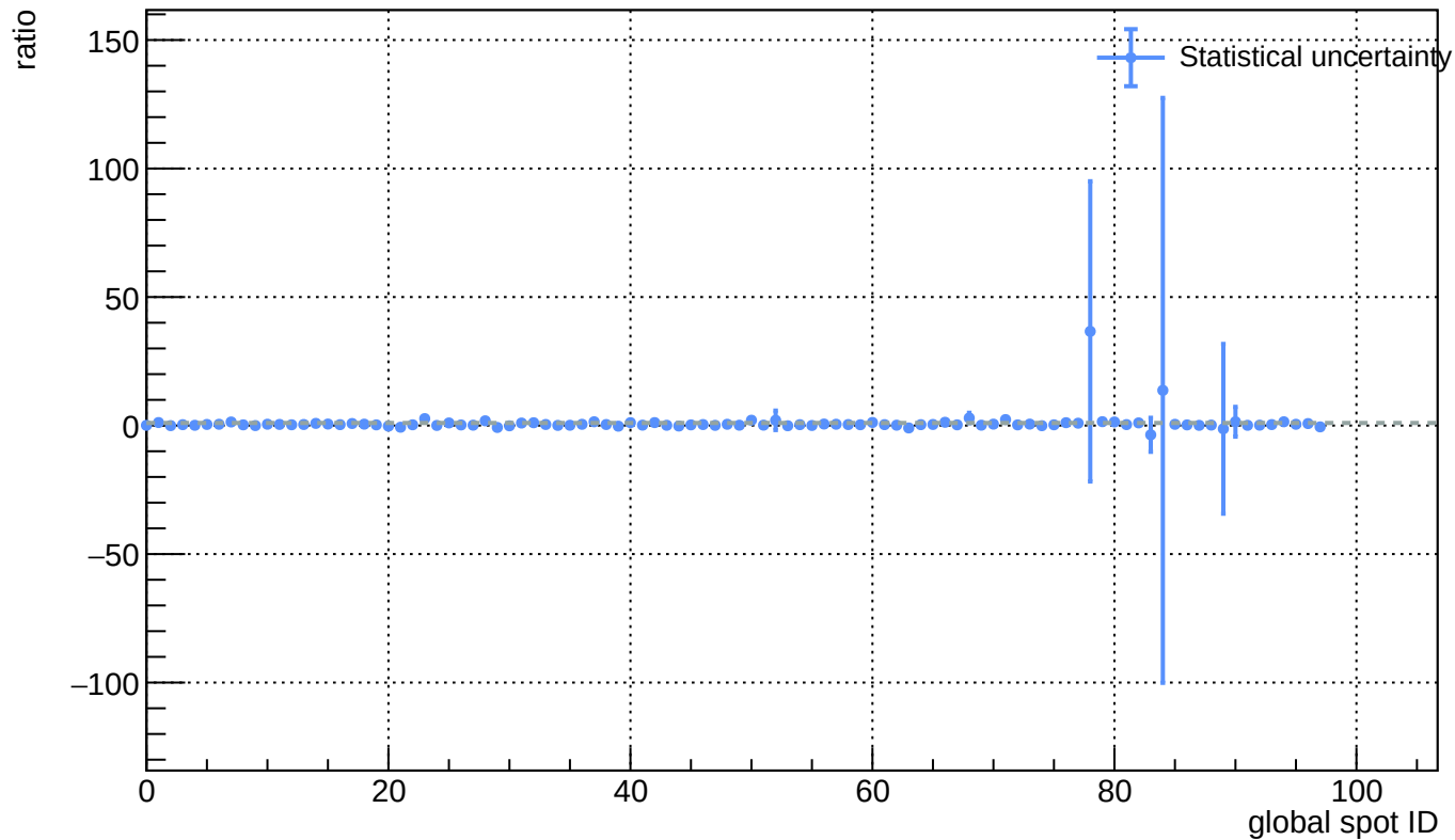
Sensor A1, T = 20 C - L(\text{ann\_125C\_5h}) / L(\text{before\_annealing})
