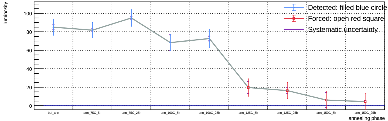
Sensor A1, T = 20 C, representative v = 58.3 V (max available) - Spot 26: luminosity vs phase
