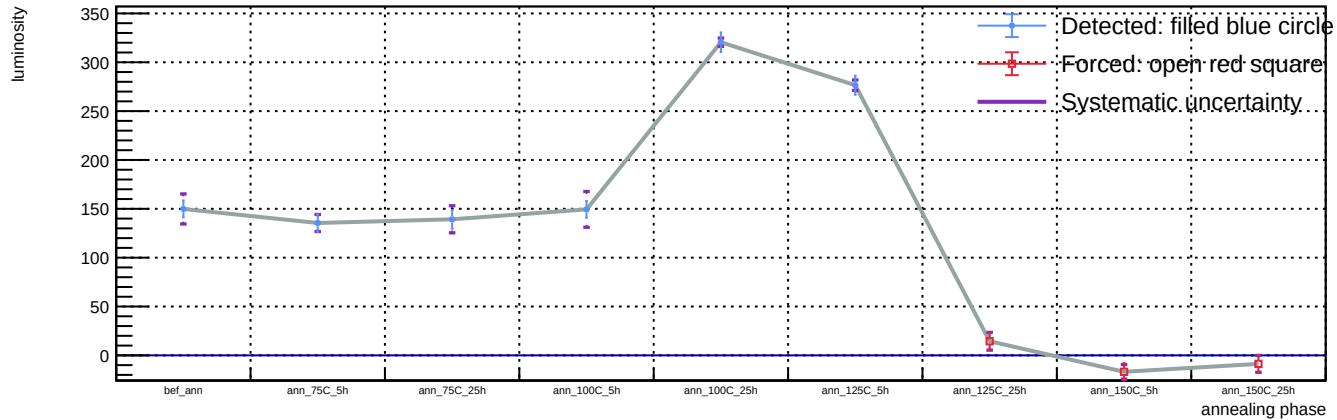
Sensor A1, T = 20 C, representative v = 58.3 V (max available) - Spot 28: luminosity vs phase
