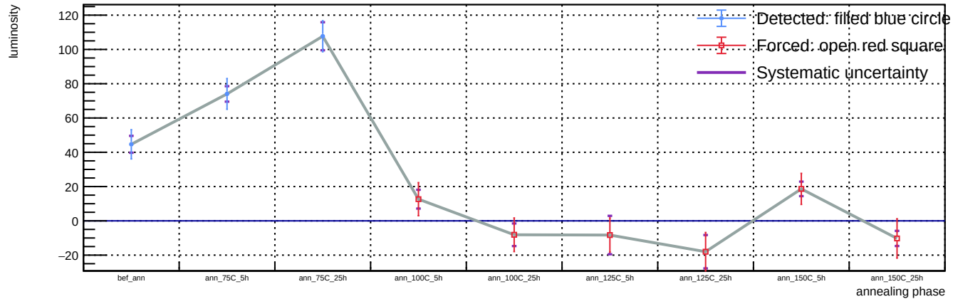
Sensor A1, T = 20 C, representative v = 58.3 V (max available) - Spot 44: luminosity vs phase
