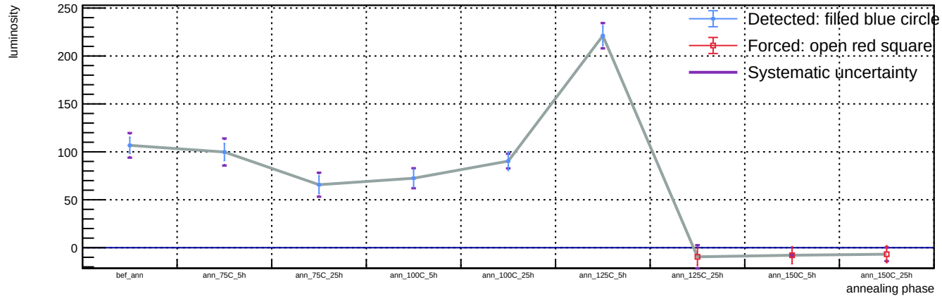
Sensor A1, T = 20 C, representative v = 58.3 V (max available) - Spot 50: luminosity vs phase
