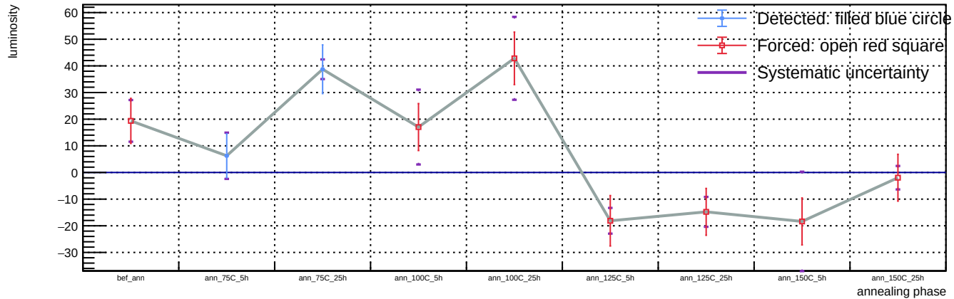
Sensor A1, T = 20 C, representative v = 58.3 V (max available) - Spot 63: luminosity vs phase
