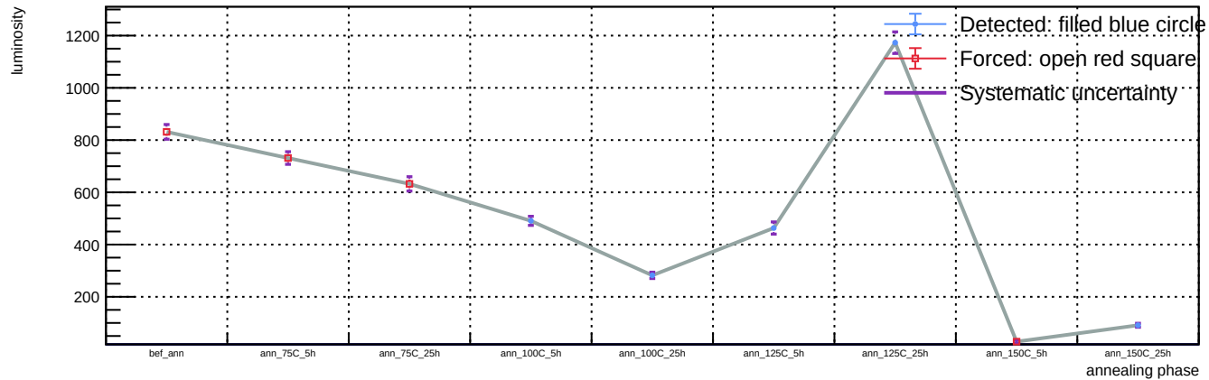
Sensor A1, T = 20 C, representative v = 58.3 V (max available) - Spot 73: luminosity vs phase
