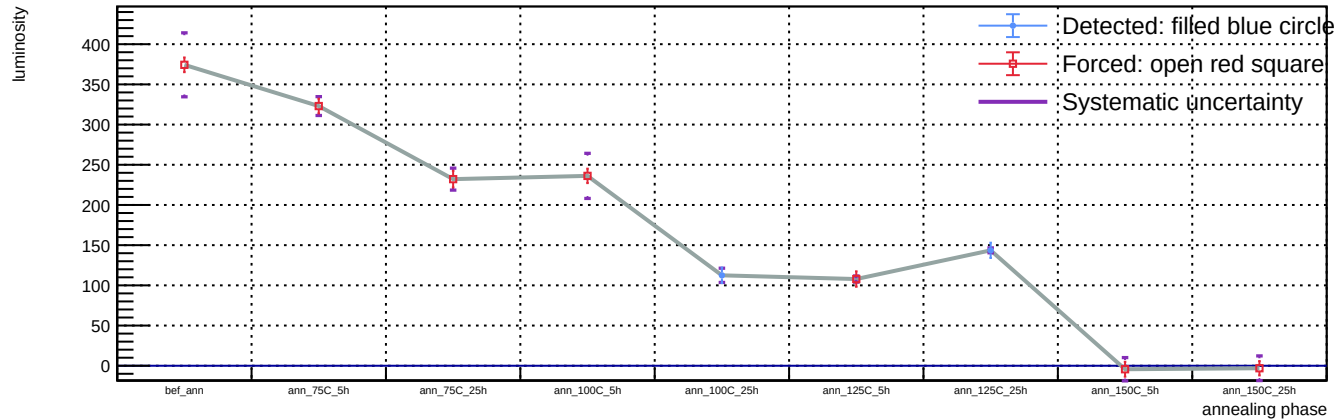
Sensor A1, T = 20 C, representative v = 58.3 V (max available) - Spot 75: luminosity vs phase
