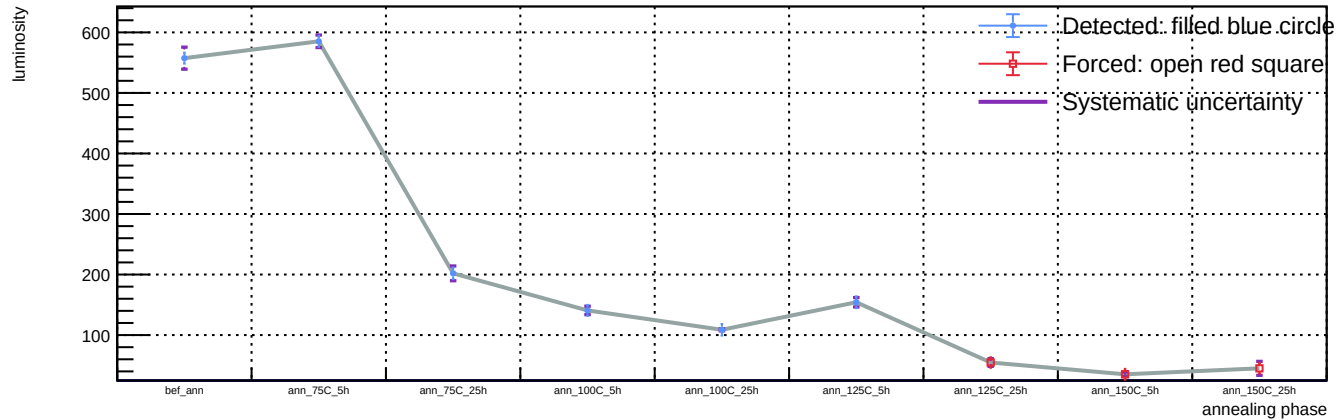
Sensor A1, T = 20 C, representative v = 58.3 V (max available) - Spot 8: luminosity vs phase
