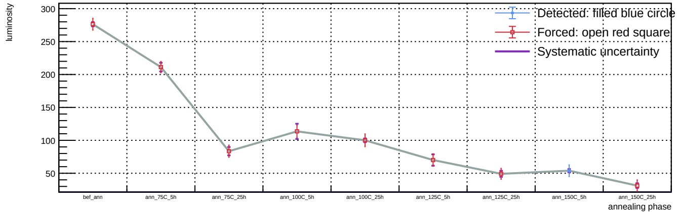
Sensor A1, T = 20 C, representative v = 58.3 V (max available) - Spot 86: luminosity vs phase
