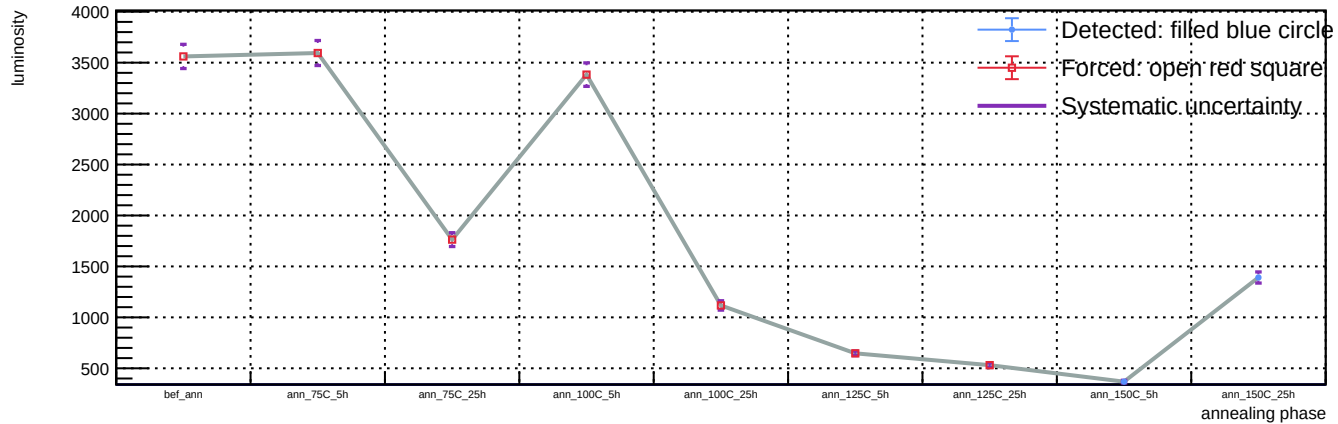
Sensor A1, T = 20 C, representative v = 58.3 V (max available) - Spot 88: luminosity vs phase
