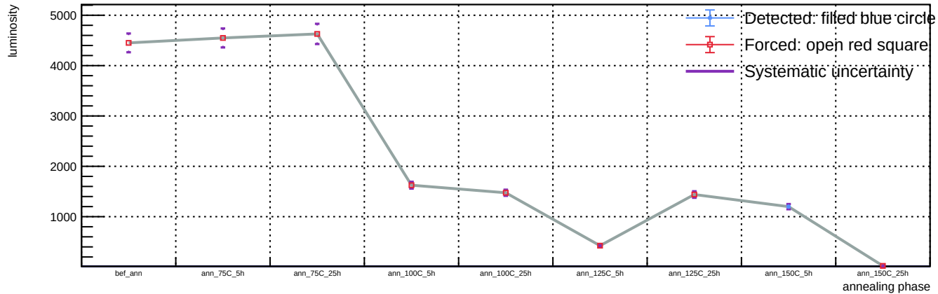
Sensor A1, T = 20 C, representative v = 58.3 V (max available) - Spot 91: luminosity vs phase
