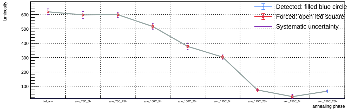
Sensor A1, T = 20 C, representative v = 58.3 V (max available) - Spot 95: luminosity vs phase
