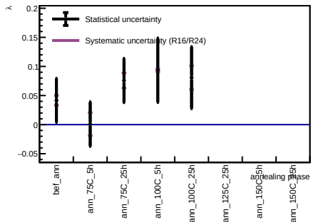
Sensor A1, v = 5 V - Spot 43
