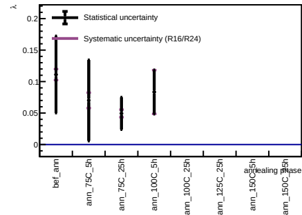
Sensor A1, v = 5 V - Spot 47
