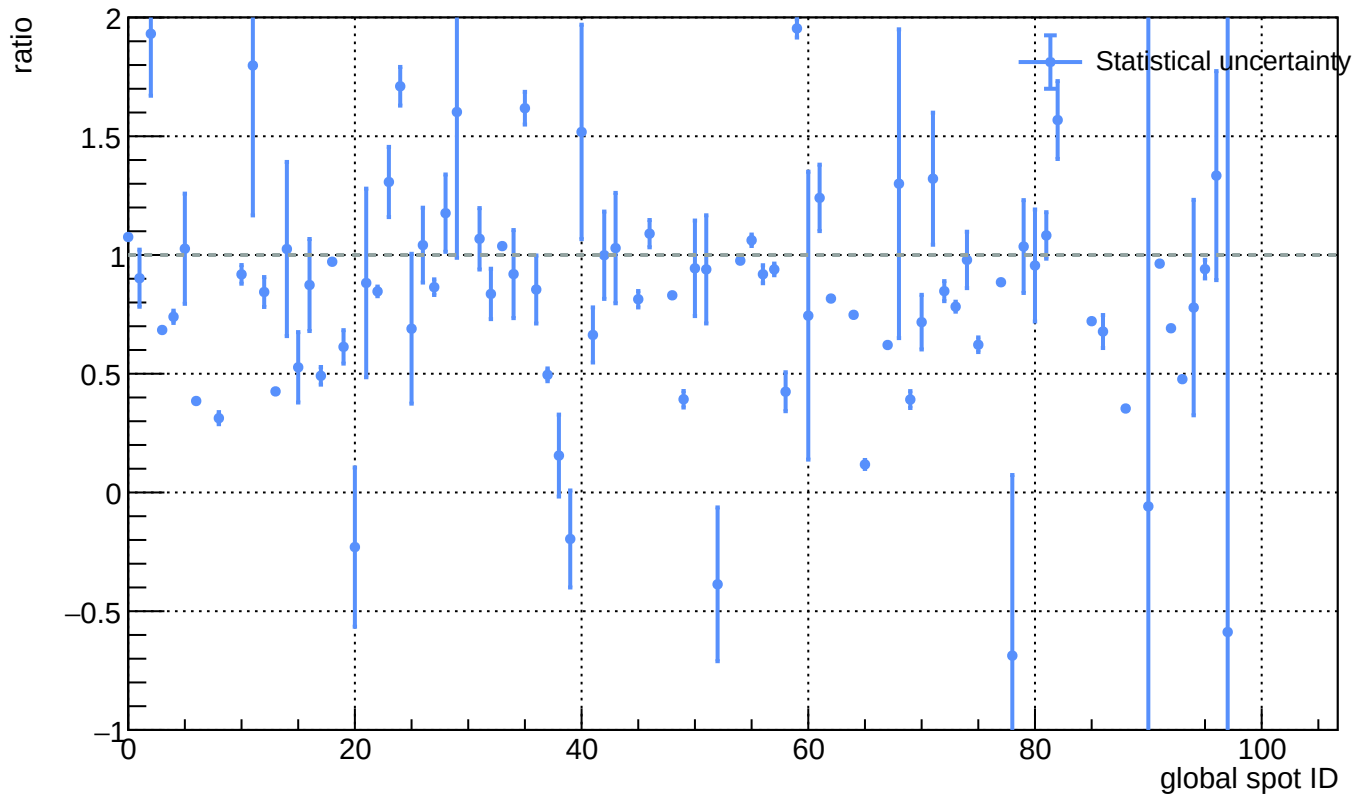
Sensor A1, v = 5 V - L(\text{ann\_75C\_25h}) / L(\text{before\_annealing})
