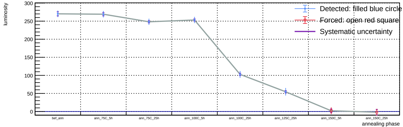
Sensor A1, v = 5 V, representative T = 23 C (max available) - Spot 10: luminosity vs phase
