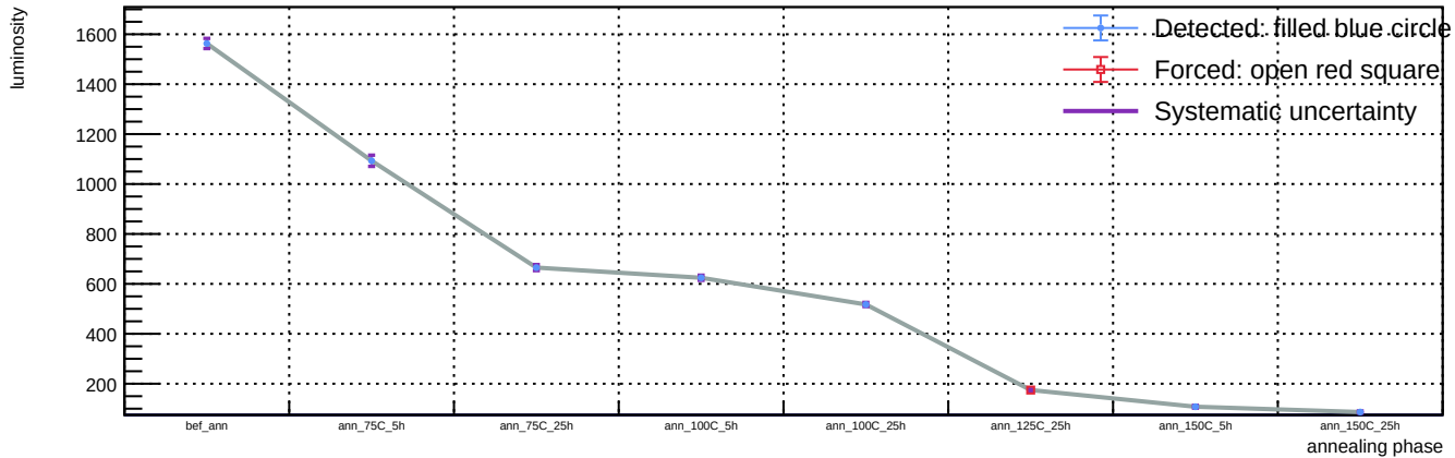
Sensor A1, v = 5 V, representative T = 23 C (max available) - Spot 13: luminosity vs phase
