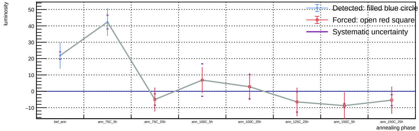
Sensor A1, v = 5 V, representative T = 23 C (max available) - Spot 20: luminosity vs phase
