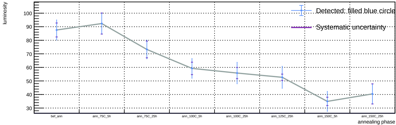
Sensor A1, v = 5 V, representative T = 23 C (max available) - Spot 32: luminosity vs phase
