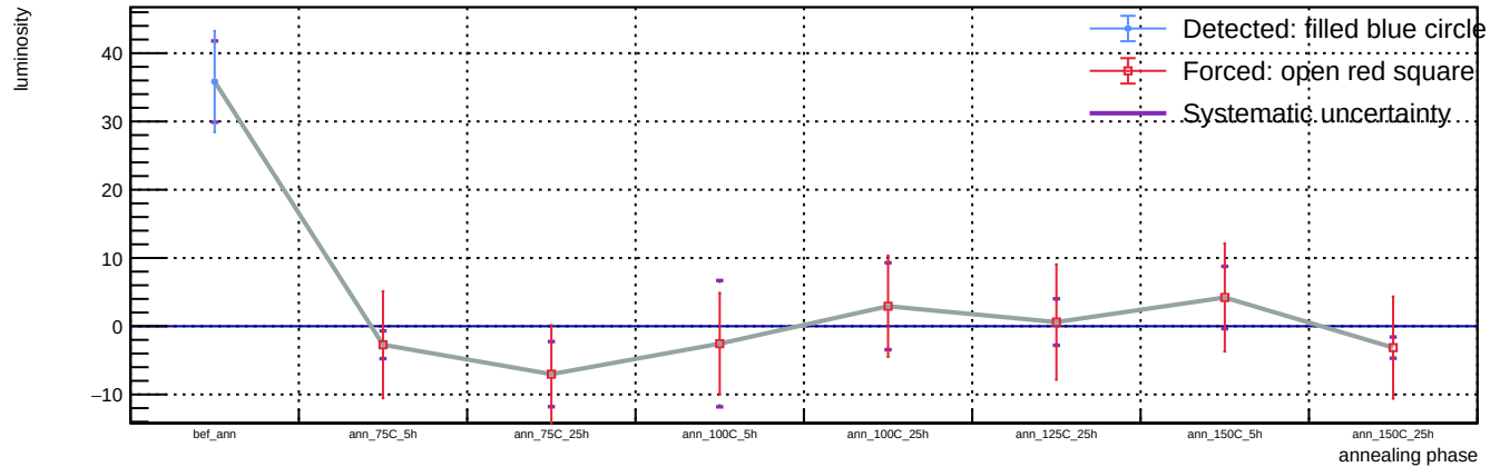
Sensor A1, v = 5 V, representative T = 23 C (max available) - Spot 39: luminosity vs phase
