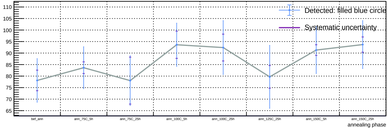
Sensor A1, v = 5 V, representative T = 23 C (max available) - Spot 42: luminosity vs phase
