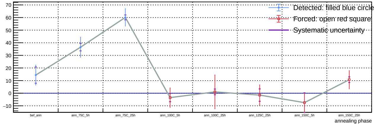
Sensor A1, v = 5 V, representative T = 23 C (max available) - Spot 44: luminosity vs phase
