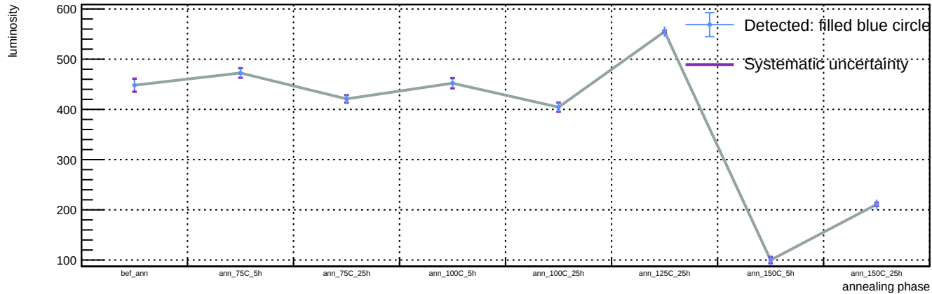
Sensor A1, v = 5 V, representative T = 23 C (max available) - Spot 57: luminosity vs phase
