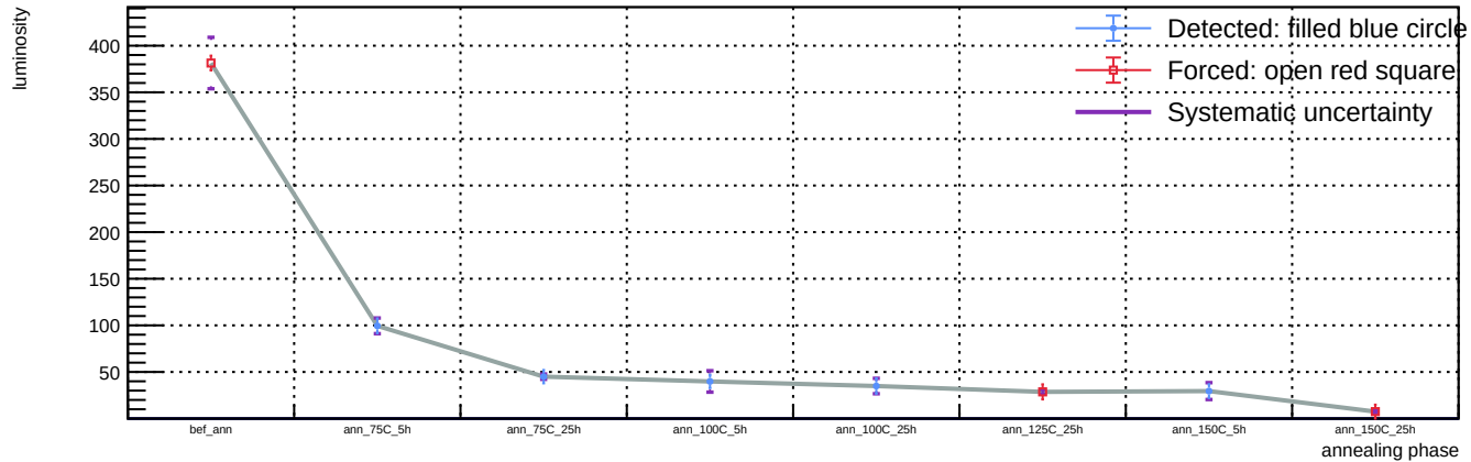
Sensor A1, v = 5 V, representative T = 23 C (max available) - Spot 65: luminosity vs phase
