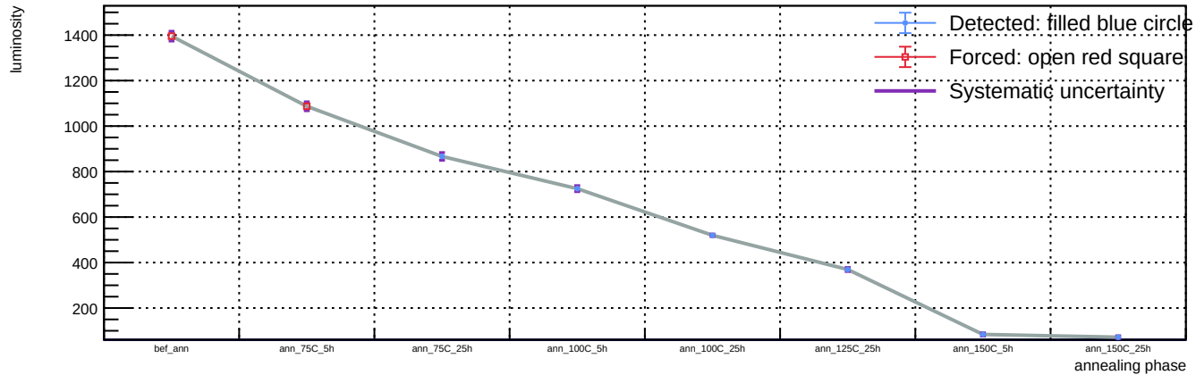
Sensor A1, v = 5 V, representative T = 23 C (max available) - Spot 67: luminosity vs phase
