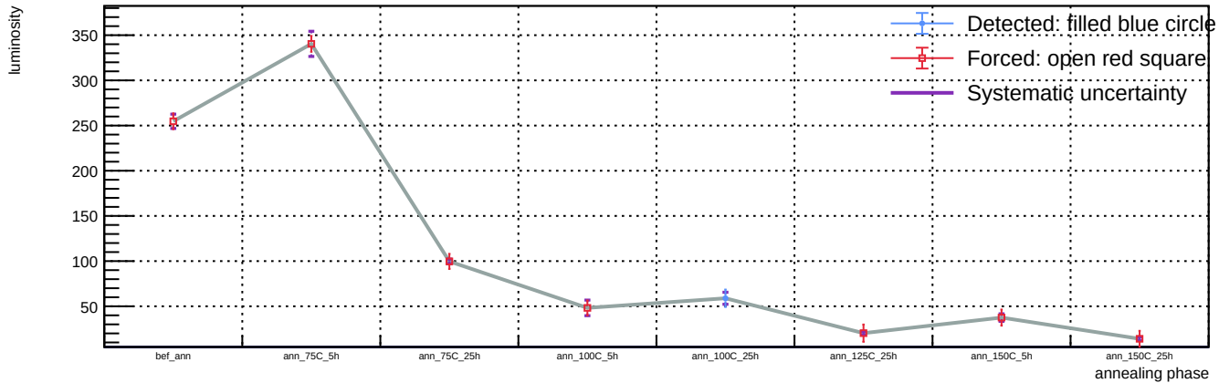
Sensor A1, v = 5 V, representative T = 23 C (max available) - Spot 69: luminosity vs phase
