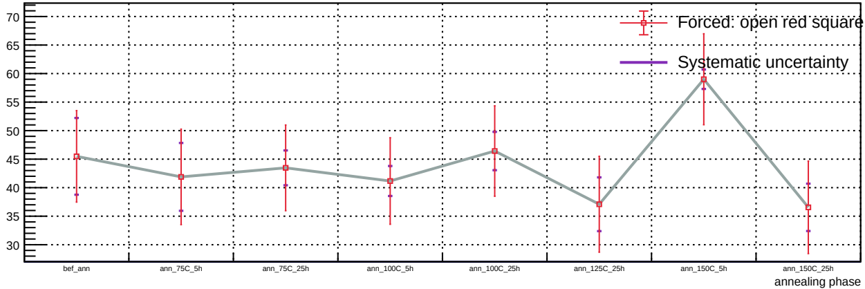
Sensor A1, v = 5 V, representative T = 23 C (max available) - Spot 80: luminosity vs phase
