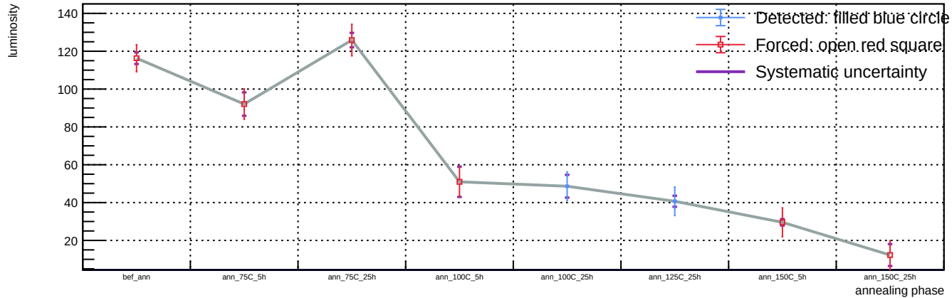
Sensor A1, v = 5 V, representative T = 23 C (max available) - Spot 81: luminosity vs phase
